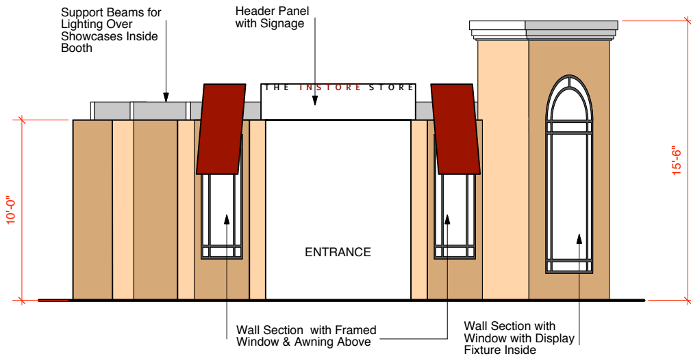
THE INSTORE STORE FRONT ELEVATION
